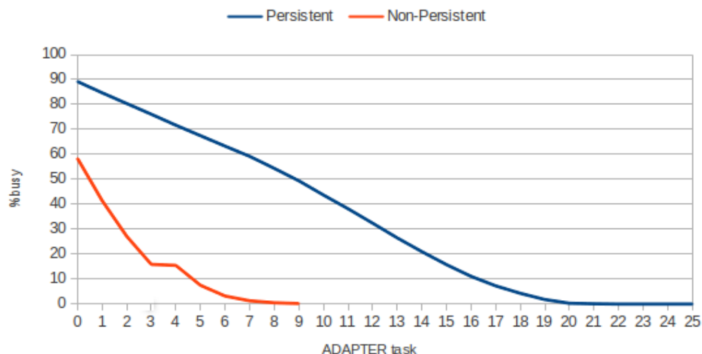
Adapter usage 2KB request/reply workload across 10 pairs of SD-RC channels
