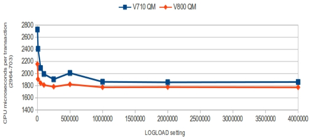
Request/Reply using 4MB messages Cost per transaction (Queue manager address space only)
