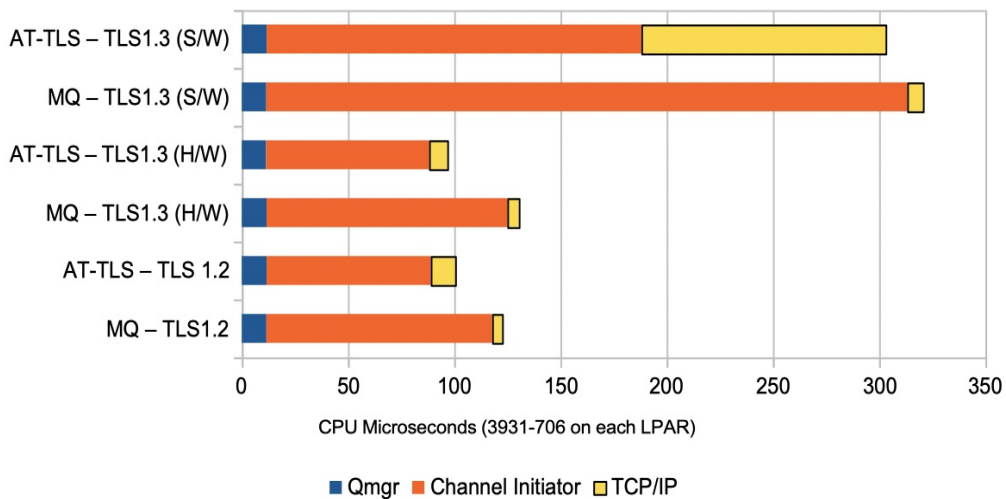
Request/Reply transport cost using 2KB non-persistent messages
