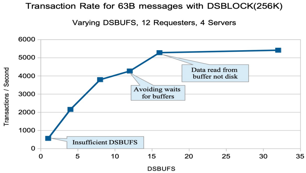
Chart: Using output from CSQE285I message to determine best DSBUFS value
