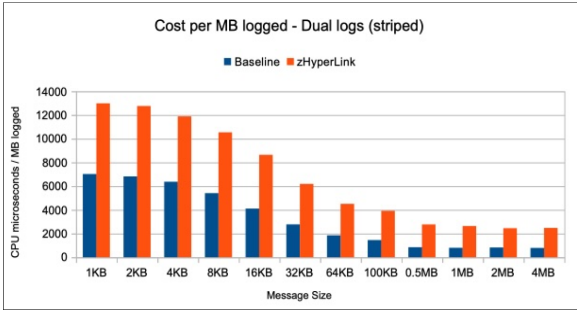
Chart: Cost per MB logged when using dual log copies (striped)
